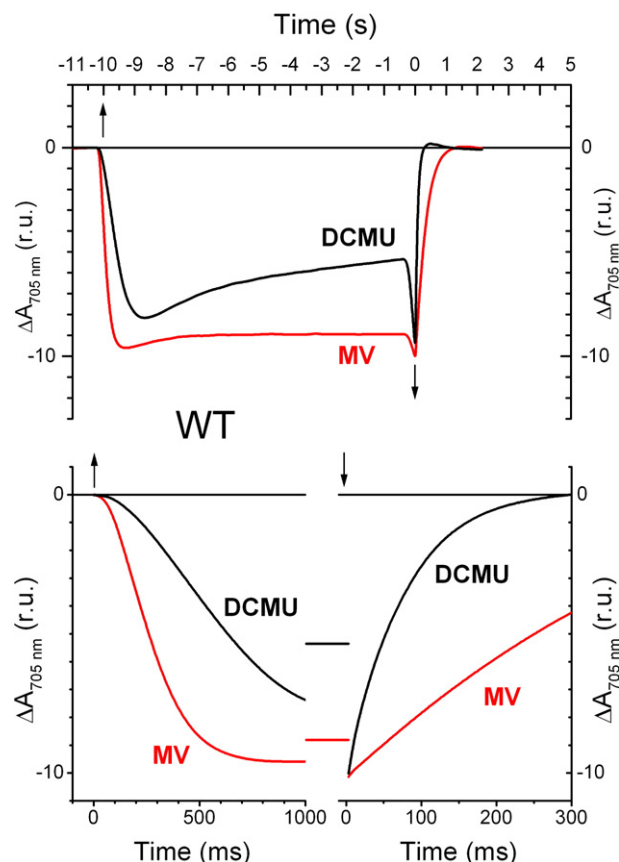
Fig. 7. Effect of 10 mM methylviologen (MV) on P_{700} oxidation–reduction kinetics measured in the presence of DCMU. The light intensity was about 50 \mu E m^{-2} s^{-1} and a saturating pulse of 200 ms was applied at the end of the illumination period to reach the full extent of P_{700}^+ .
