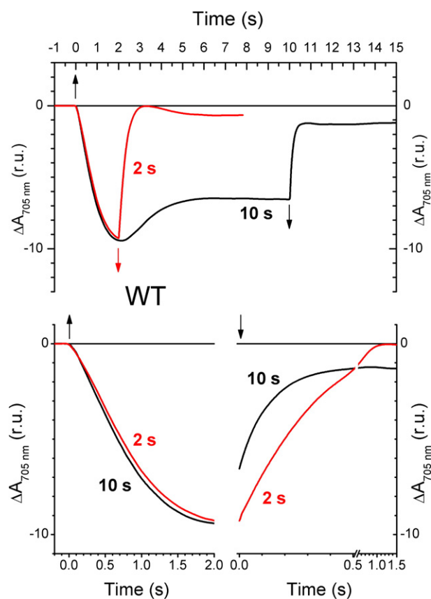
Fig. 3. Effect of the light duration on the kinetics of P_{700}^+ reduction in the dark, followed at 705 nm and induced by a 2 s or 10 s light pulse in WT algae treated with 10\text{ }\mu\text{M} DCMU. In this experiment and those shown in subsequent figures, HA ( 1\text{ mM} ) was present.
